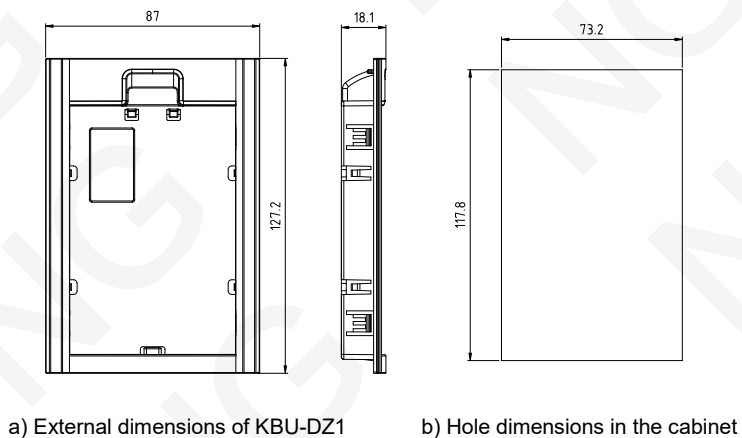
Fig. 2-6 External dimensions of KBU-DZ1 and cabinet hole dimensions
