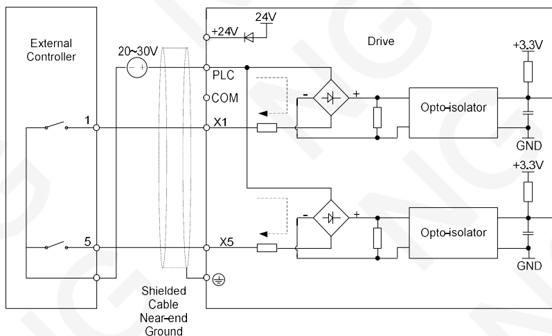
Fig. 3-30 External power supply dry contact
