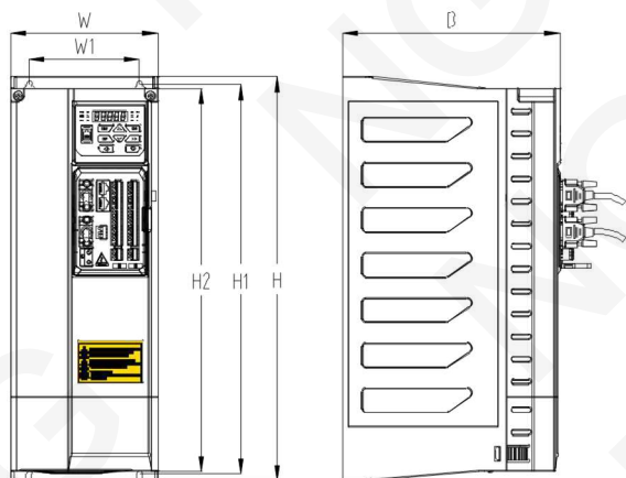
b) NG80P-4T15GB~NG80P-4T37G(B)
