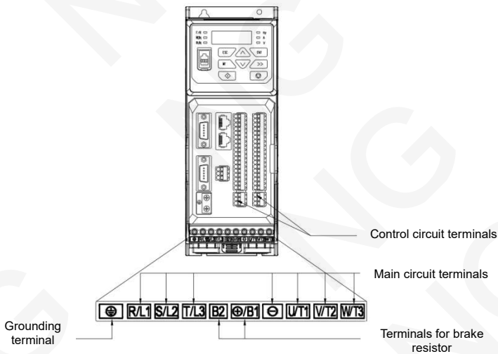
Fig. 3-22 Terminal configuration
