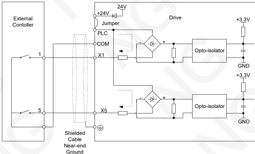
Fig. 3-29 Internal power supply dry contact
