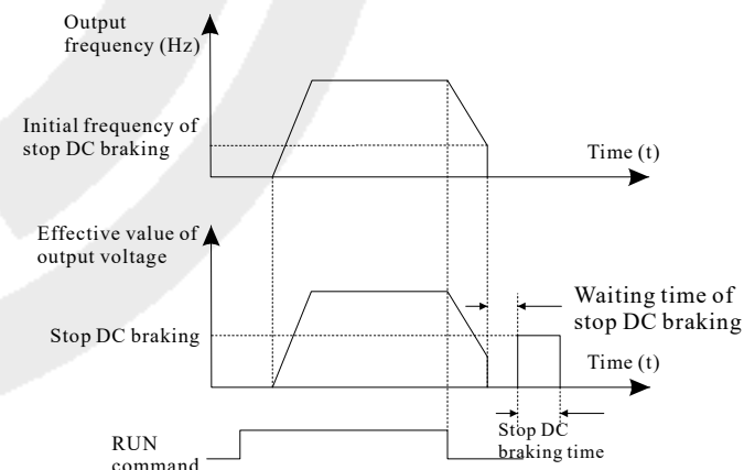
Figure 6-4 The stop DC braking process
