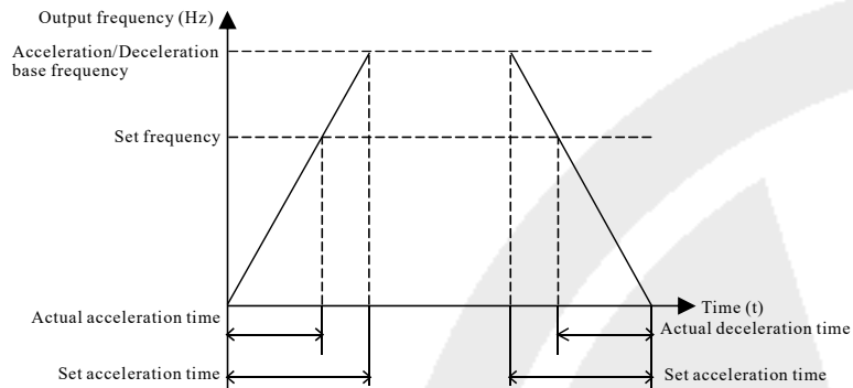
Figure 6-1 Acceleration/Deceleration time
