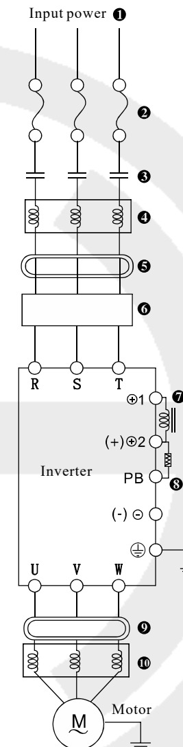
Figure3-2 Peripheral device wiring diagram
