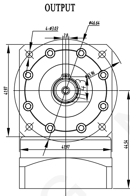
SHAFT OUTPUT 22MM
